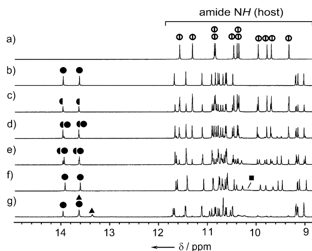
Figure 3. Parts of the ^1\text{H} NMR spectra (700 MHz) of 3 (0.5 mM in \text{CDCl}_3 ; [\text{D}_6]\text{DMSO} = 99:1 ( v/v )) at 298 K in the presence of a) 0 equiv of guest; b) 2 equiv of D/L\text{-}2 ; c) 0.5 equiv; d) 1 equiv; e) 1.5 equiv; and f) 2 equiv of L\text{-}2 ; g) 1 equiv of L\text{-}2 and 3 equiv of L\text{-}4 . For 3\text{-}(2\text{-}D;2\text{-}L) (b) signals of the carboxylic acid protons of 2 in the matching helices are denoted with full black circles. For 3\text{-}(2\text{-}L)_2 (c–g) signals of the carboxylic acid protons of L\text{-}2 in the M helix (matching) are marked with half-black circles when the P helix is empty, and with black circles when the P helix also hosts a guest; signals of the carboxylic acid protons of L\text{-}2 in the P helix (mismatching) are marked with a black square. It should be noted that the two mismatching acid resonances are at coalescence at this temperature. For 3\text{-}(2\text{-}L;4\text{-}L) , signals of the carboxylic acid protons of L\text{-}2 in the M helix (matching) are marked with black circles and carboxylic acid protons of L\text{-}4 in the P helix (matching) are denoted with black triangles.
