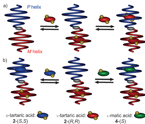
Figure 2. Schematic representation of the encapsulation of a) two molecules of the L -enantiomer of tartaric acid and b) a racemic mixture of D - and L -tartaric acid (left equilibrium) and a mixture of L -tartaric acid and L -malic acid (right equilibrium) in host 3 , which possesses two cavities of opposite handedness. P and M handedness are denoted in blue and red, respectively. The inversion center controlling the stereochemistry of 3 is colored in light grey. The golden balls stand for the hydroxy groups of the guests. Red-in-blue and blue-in-red complexes are mismatching complexes.
